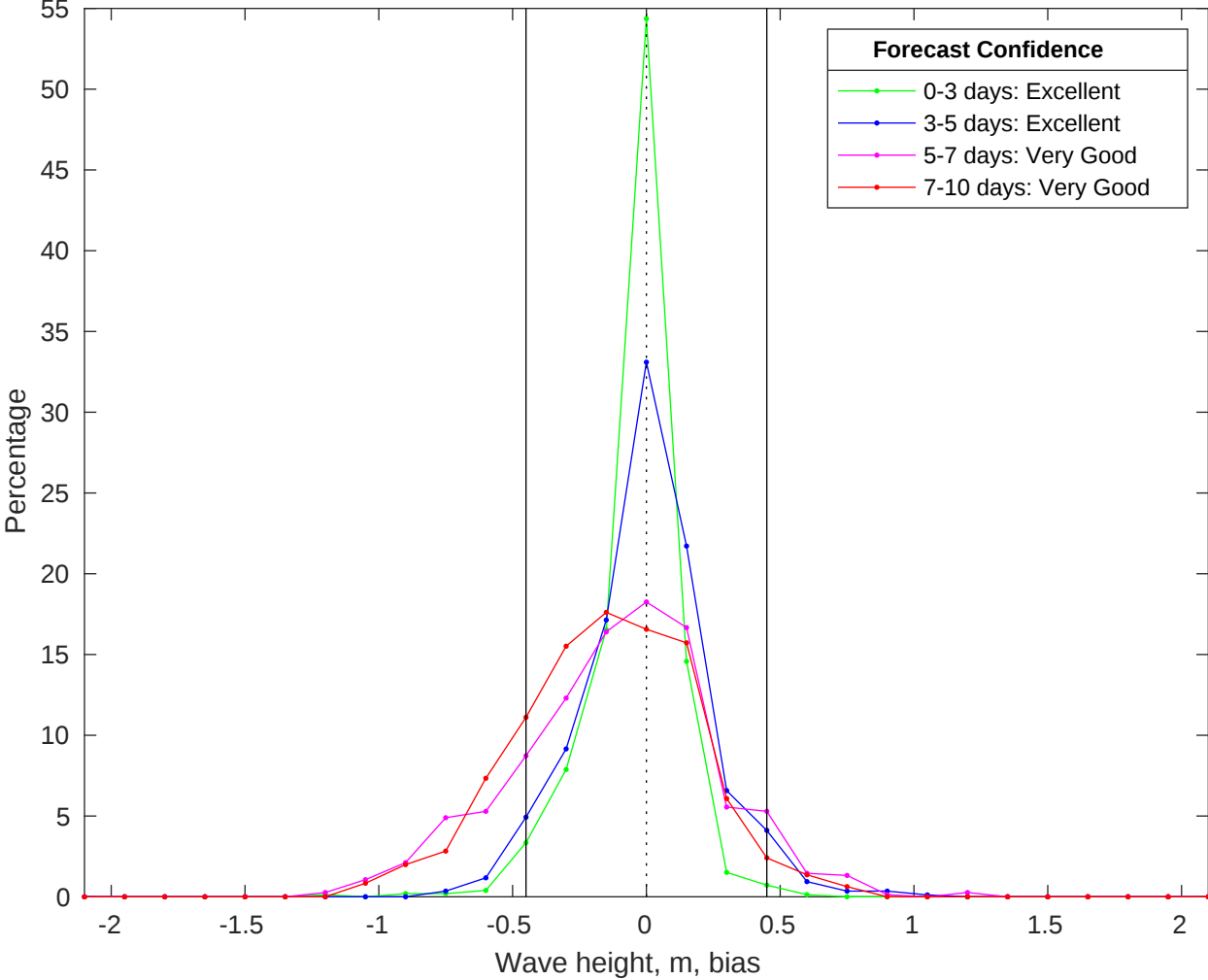
NDBC 41004 vs CMEMS Waves Bias Histogram: 05-Jun-2025
