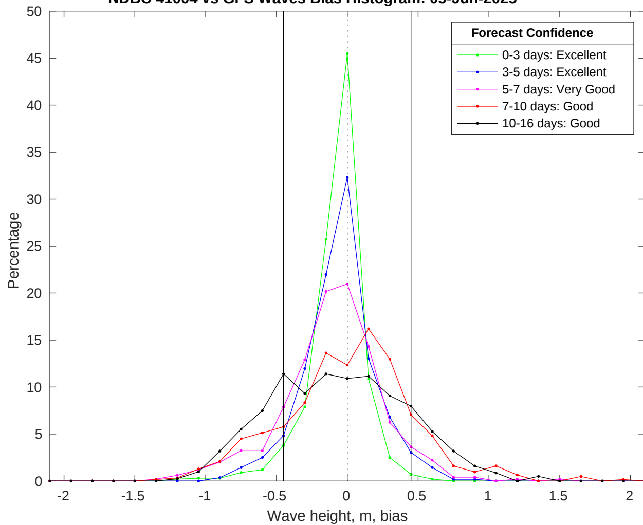
NDBC 41004 vs GFS Waves Bias Histogram: 05-Jun-2025
