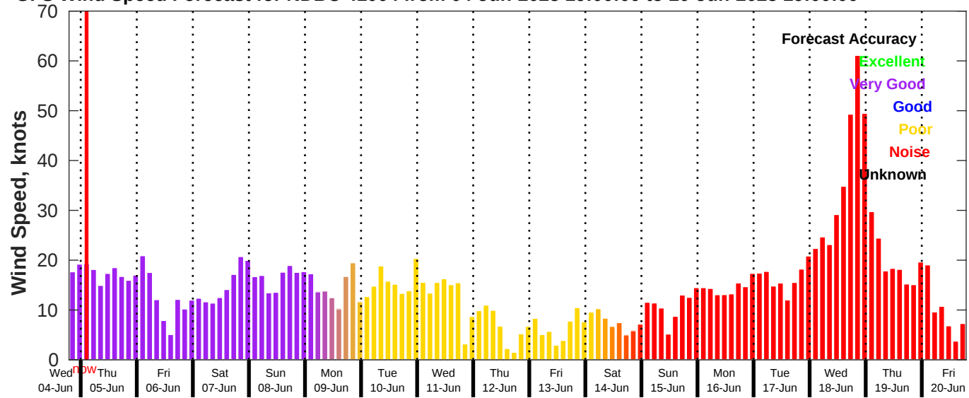
GFS Wind Speed Forecast for NDBC 41004 from 04-Jun-2025 19:00:00 to 20-Jun-2025 19:00:00
