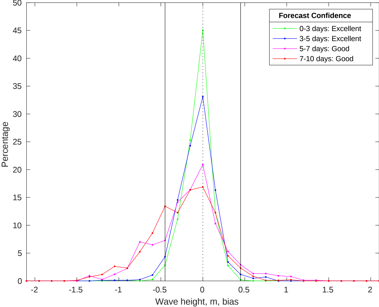
NDBC 41013 vs CMEMS Waves Bias Histogram: 05-Jun-2025
