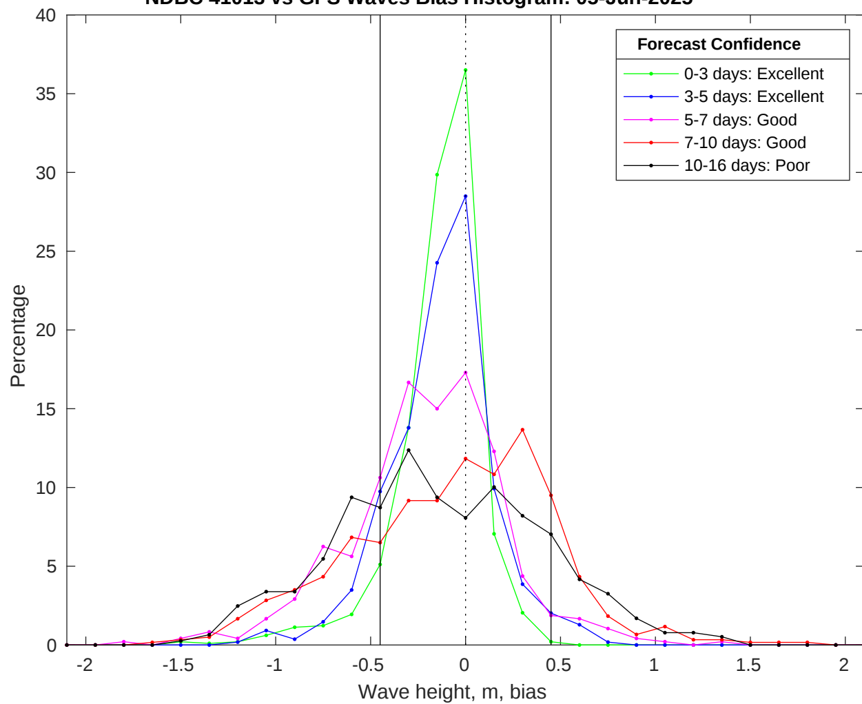
NDBC 41013 vs GFS Waves Bias Histogram: 05-Jun-2025
