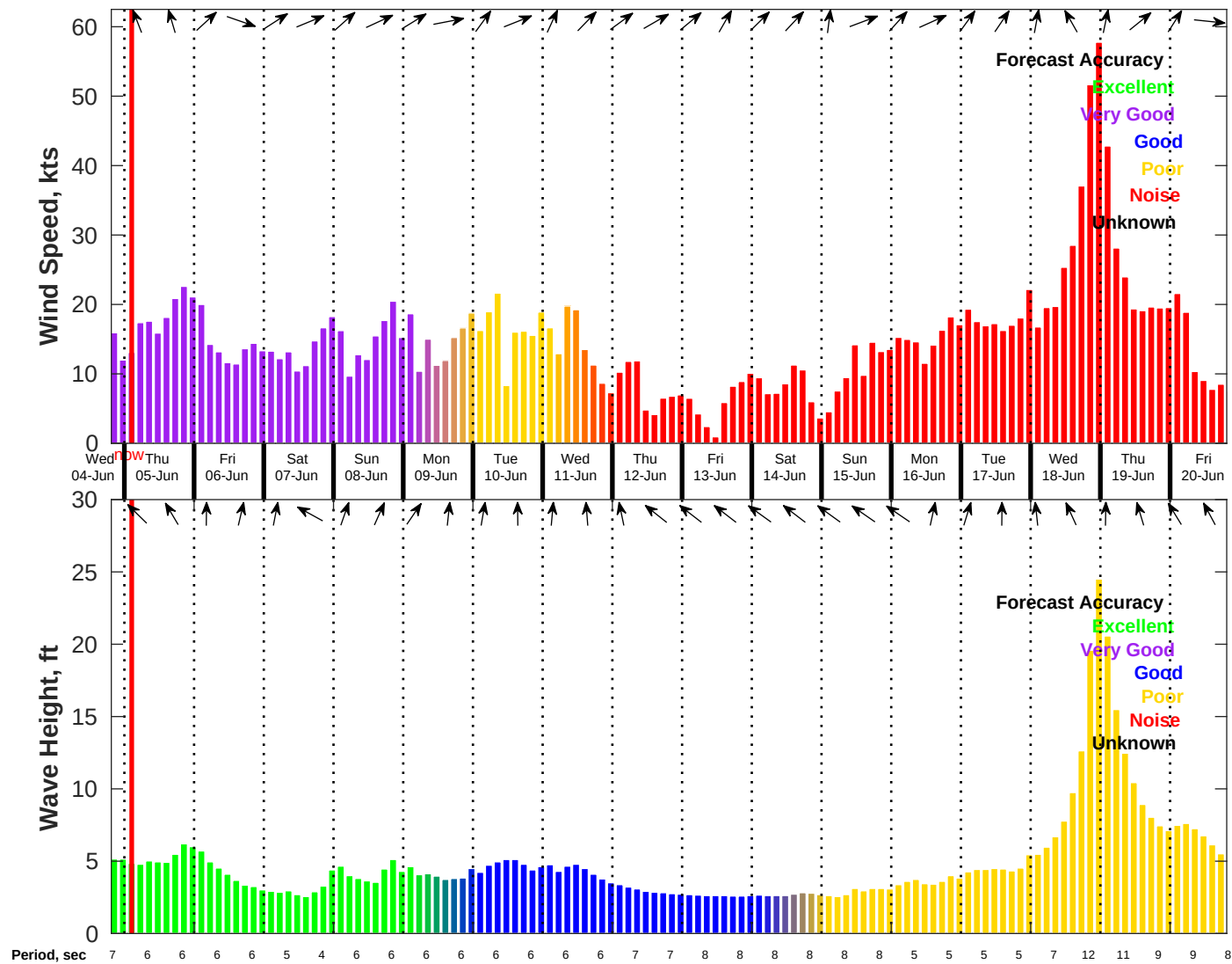
Wind & Wave Forecast for NDBC 41013 from 04-Jun-2025 19:00:00 to 20-Jun-2025 19:00:00
