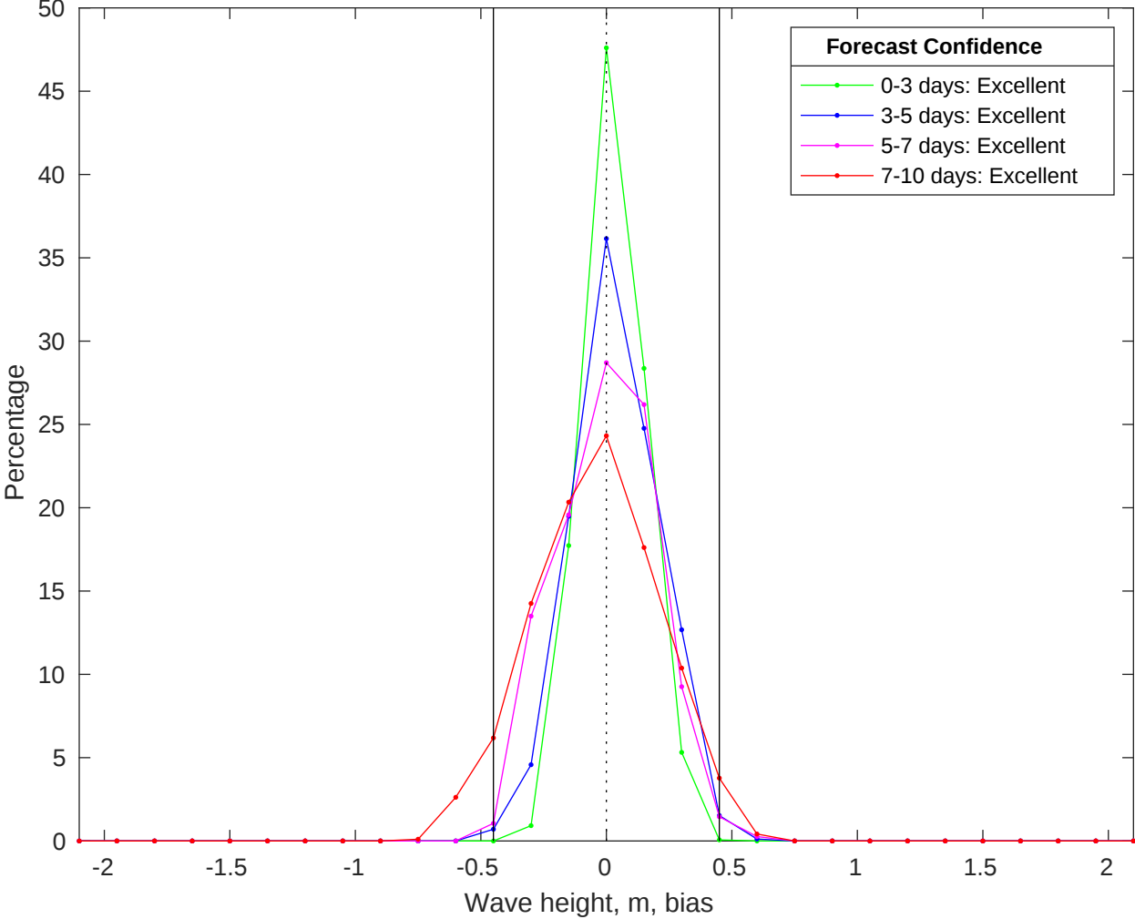
NDBC 41040 vs CMEMS Waves Bias Histogram: 05-Jun-2025
