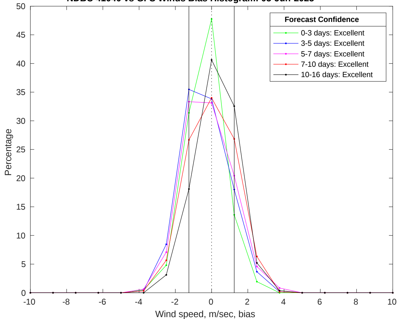
NDBC 41040 vs GFS Winds Bias Histogram: 05-Jun-2025
