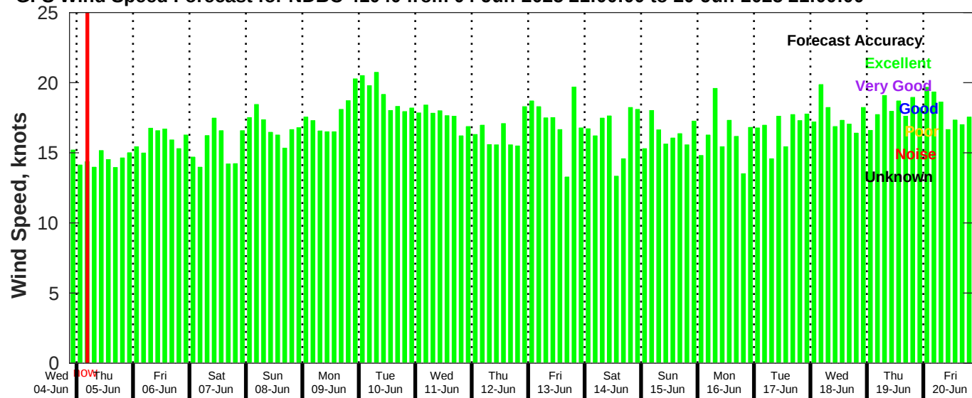
GFS Wind Speed Forecast for NDBC 41040 from 04-Jun-2025 21:00:00 to 20-Jun-2025 21:00:00
