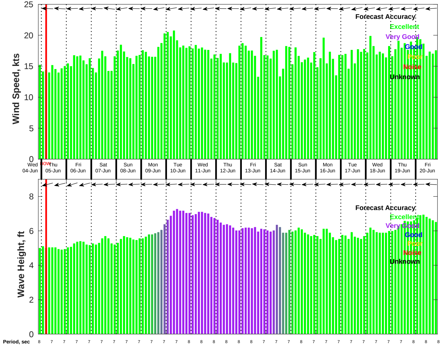
Wind & Wave Forecast for NDBC 41040 from 04-Jun-2025 21:00:00 to 20-Jun-2025 21:00:00
