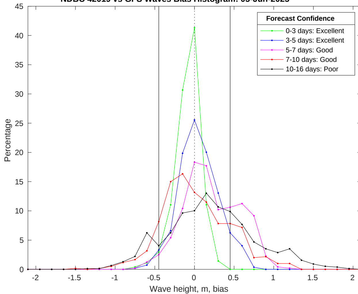
NDBC 42019 vs GFS Waves Bias Histogram: 05-Jun-2025
