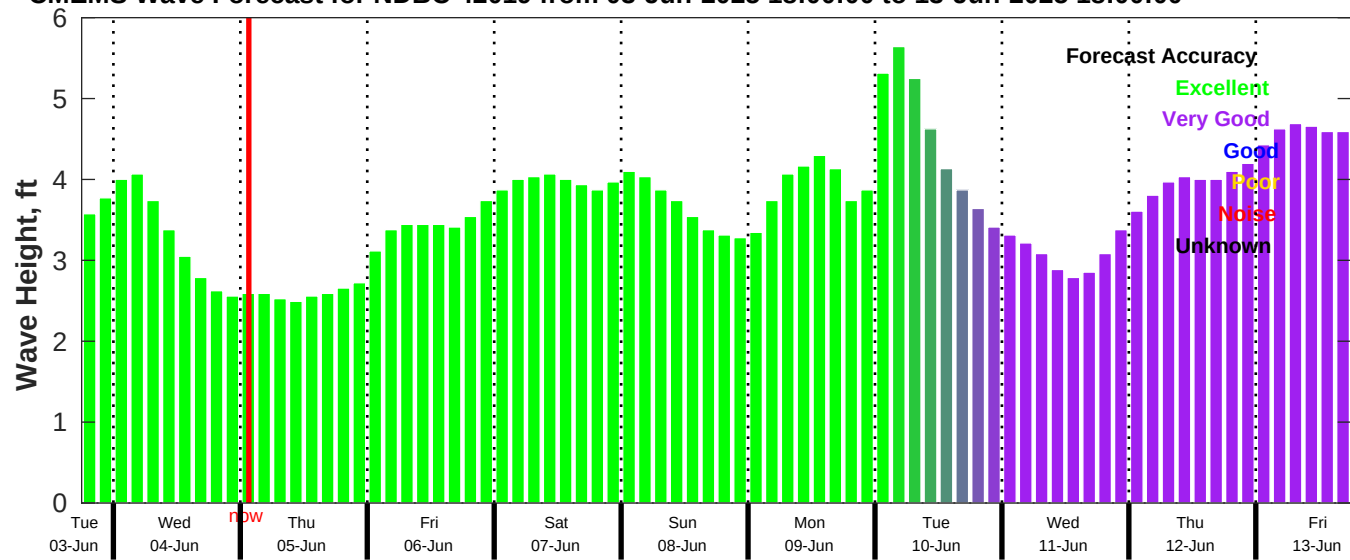
CMEMS Wave Forecast for NDBC 42019 from 03-Jun-2025 18:00:00 to 13-Jun-2025 18:00:00
