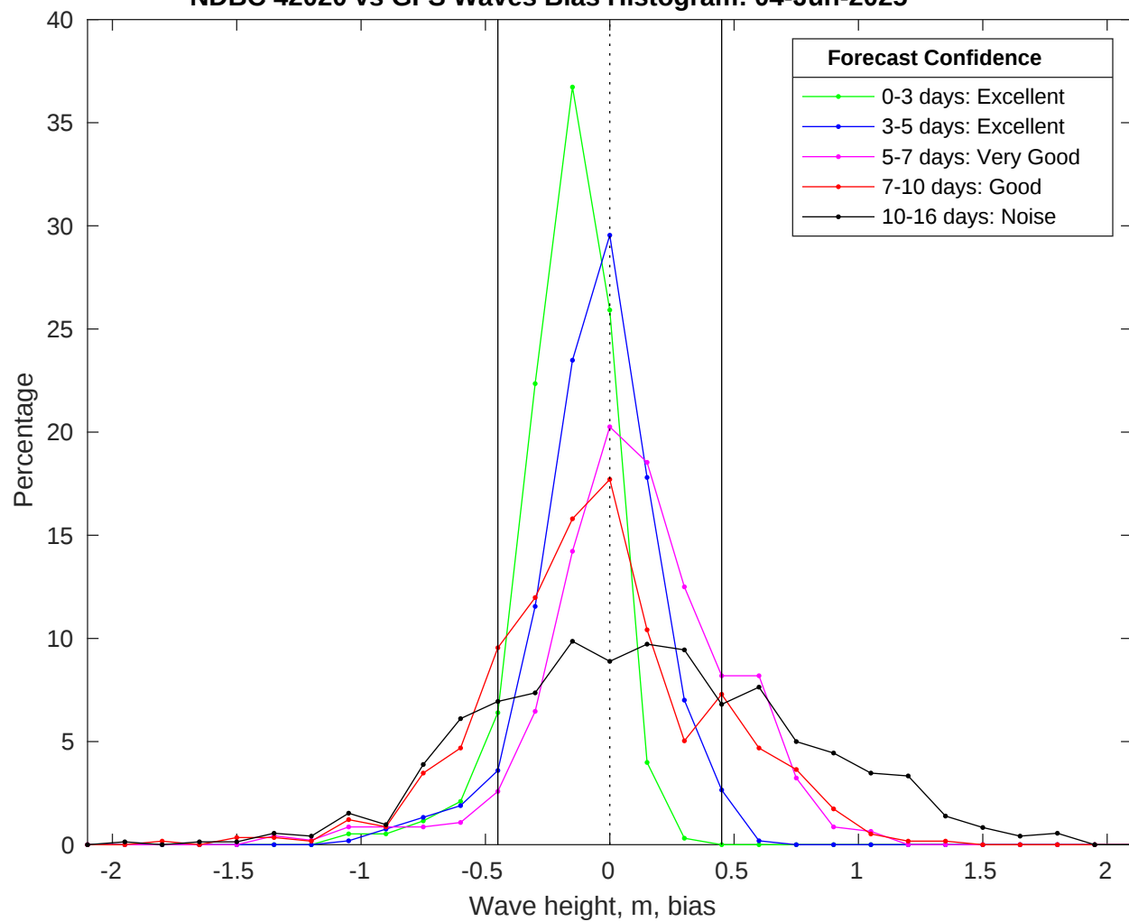
NDBC 42020 vs GFS Waves Bias Histogram: 04-Jun-2025
