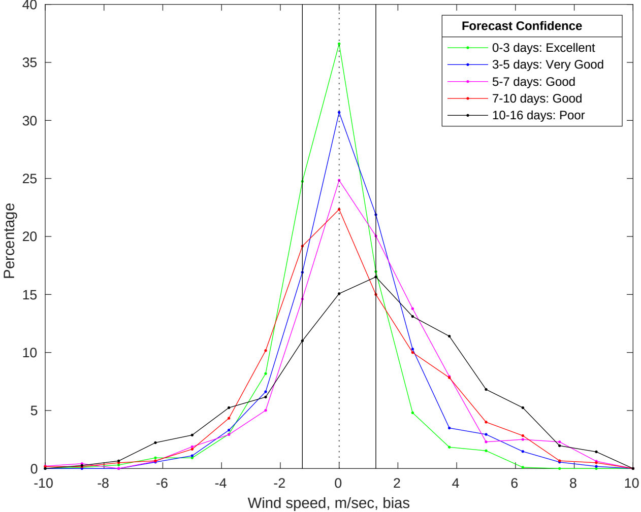
NDBC 42020 vs GFS Winds Bias Histogram: 05-Jun-2025
