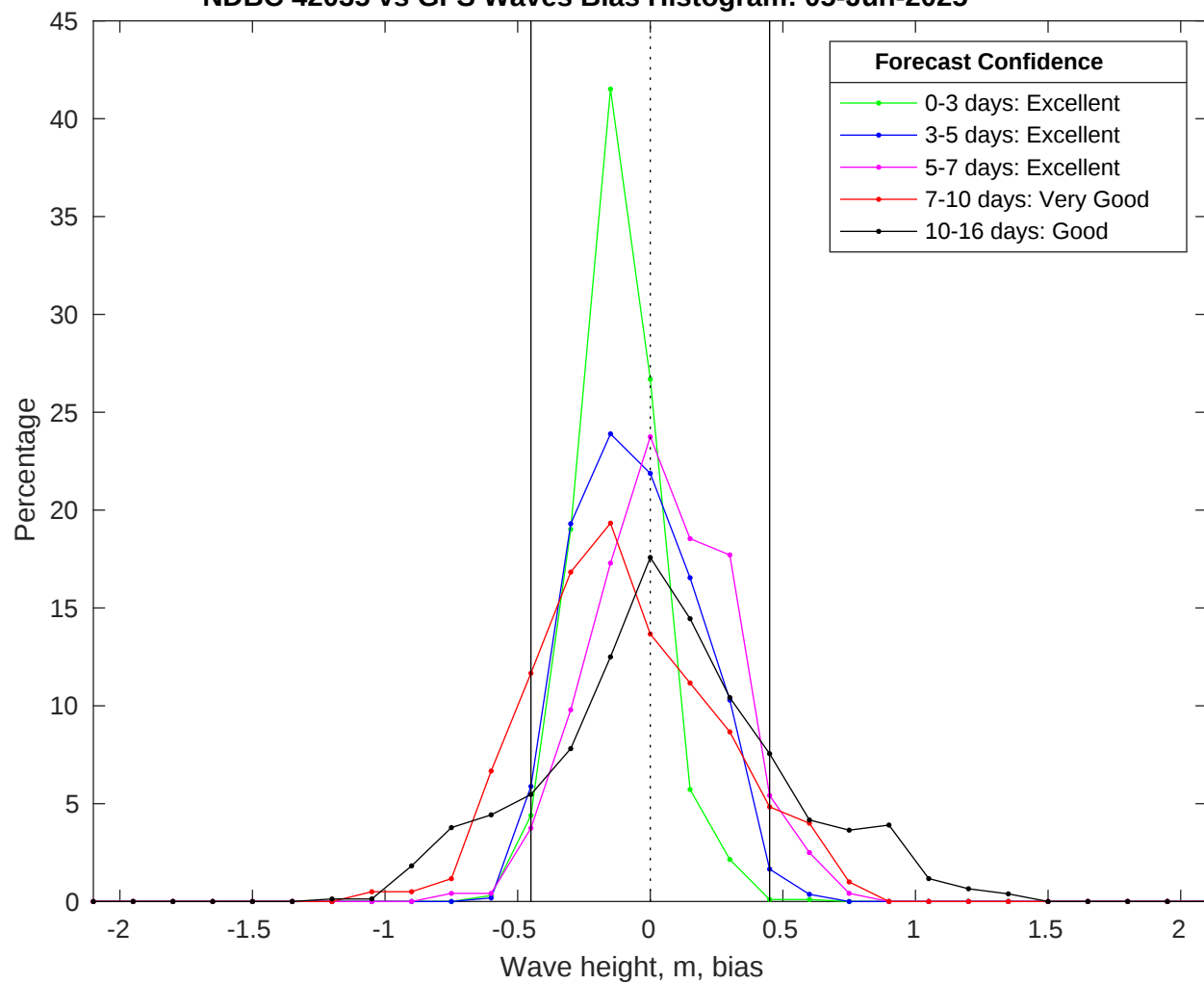
NDBC 42035 vs GFS Waves Bias Histogram: 05-Jun-2025
