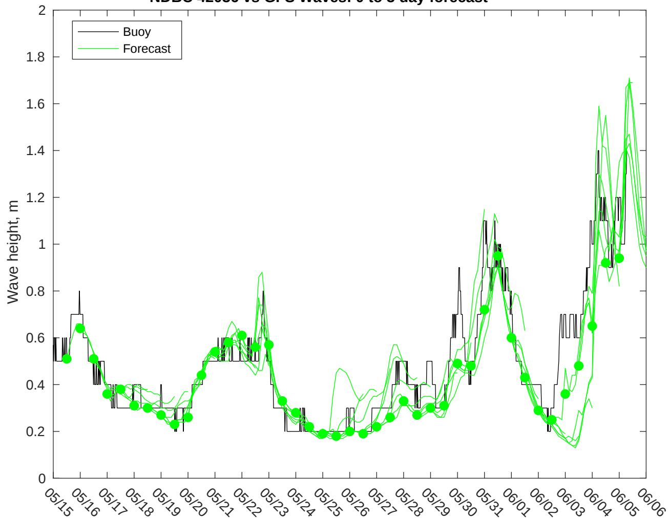
NDBC 42036 vs GFS Waves: 0 to 3 day forecast
