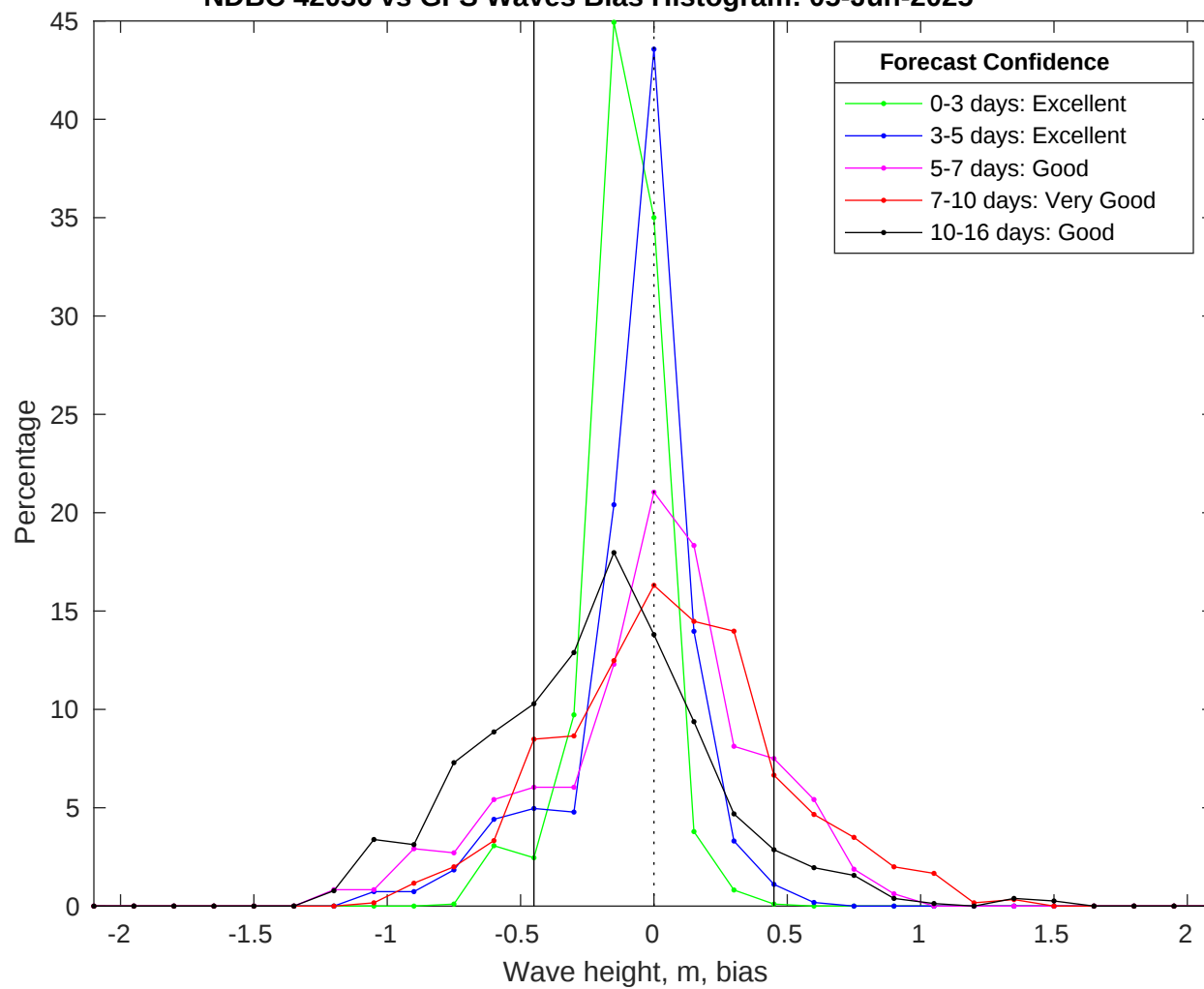
NDBC 42036 vs GFS Waves Bias Histogram: 05-Jun-2025
