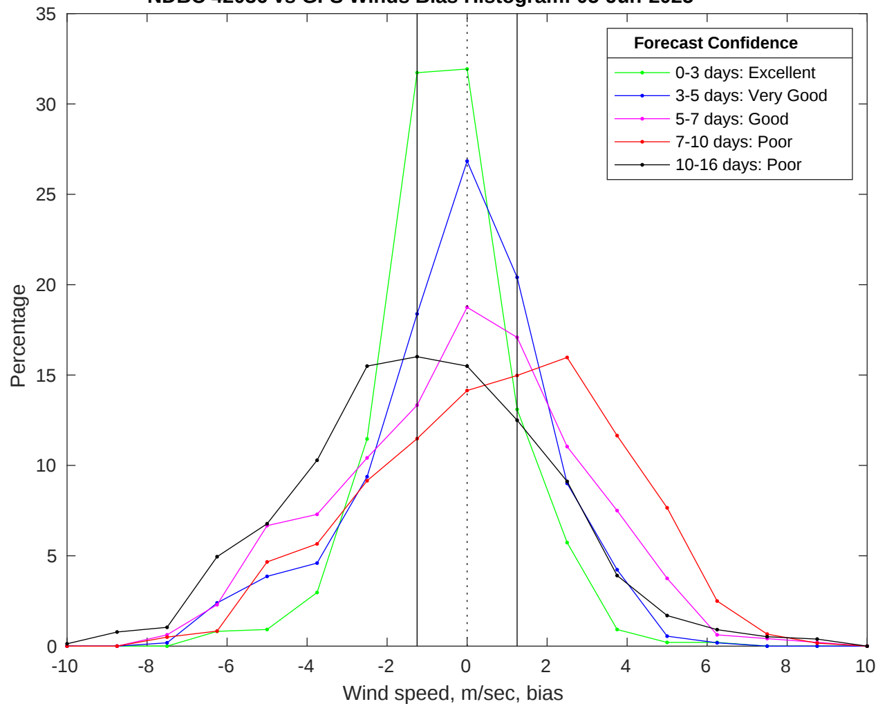
NDBC 42036 vs GFS Winds Bias Histogram: 05-Jun-2025
