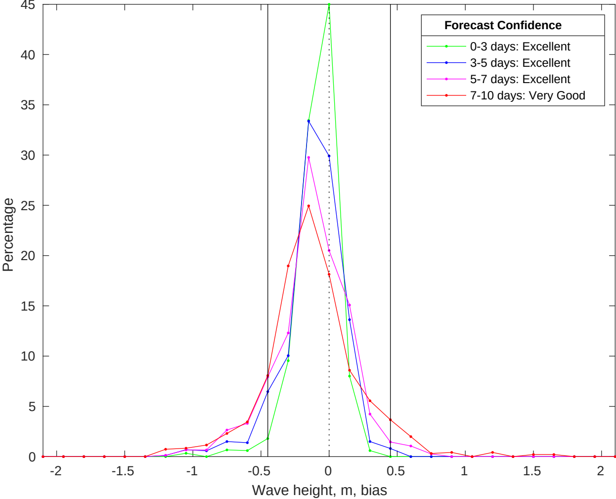
NDBC 42040 vs CMEMS Waves Bias Histogram: 05-Jun-2025
