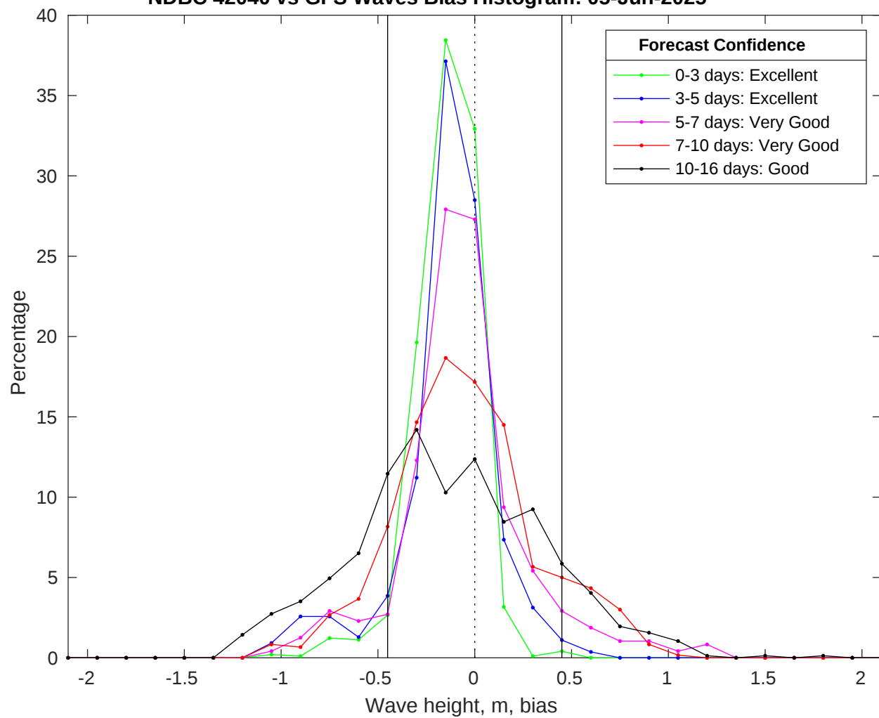
NDBC 42040 vs GFS Waves Bias Histogram: 05-Jun-2025
