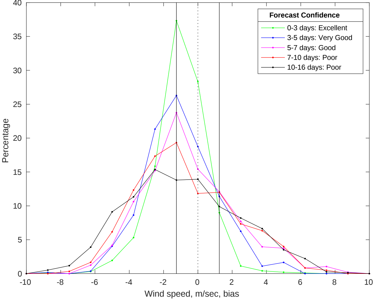
NDBC 42040 vs GFS Winds Bias Histogram: 05-Jun-2025
