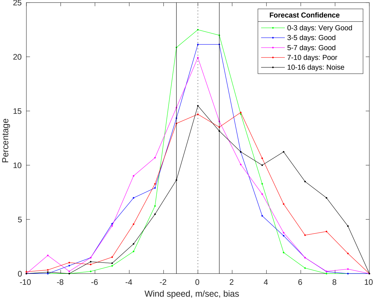
NDBC 46011 vs GFS Winds Bias Histogram: 05-Jun-2025
