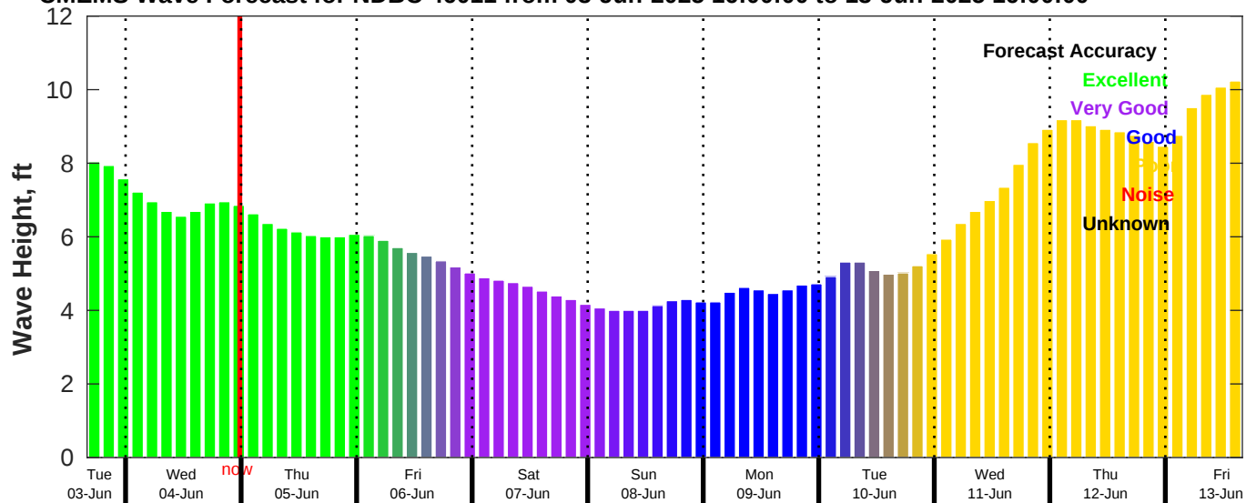
CMEMS Wave Forecast for NDBC 46011 from 03-Jun-2025 16:00:00 to 13-Jun-2025 16:00:00
