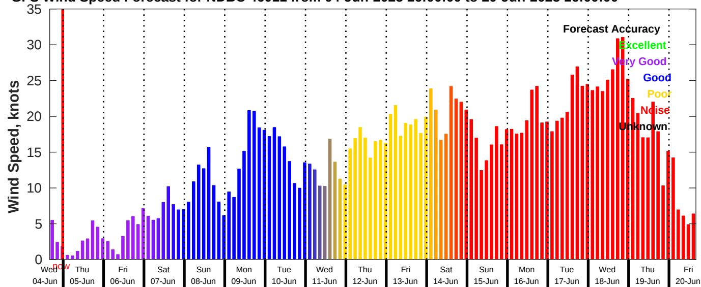
GFS Wind Speed Forecast for NDBC 46011 from 04-Jun-2025 16:00:00 to 20-Jun-2025 16:00:00
