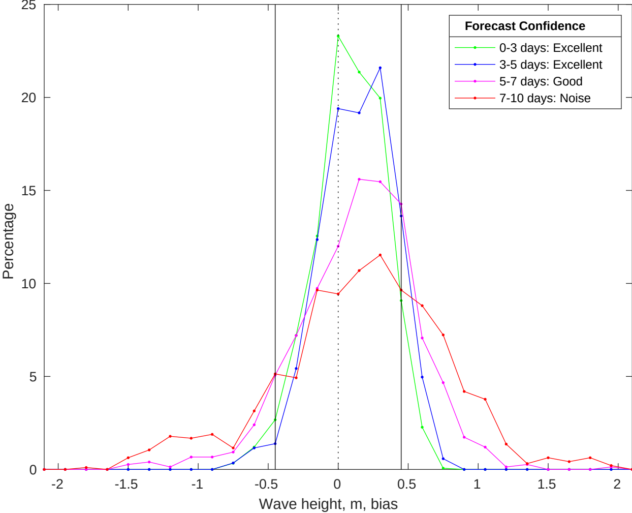
NDBC 46028 vs CMEMS Waves Bias Histogram: 05-Jun-2025
