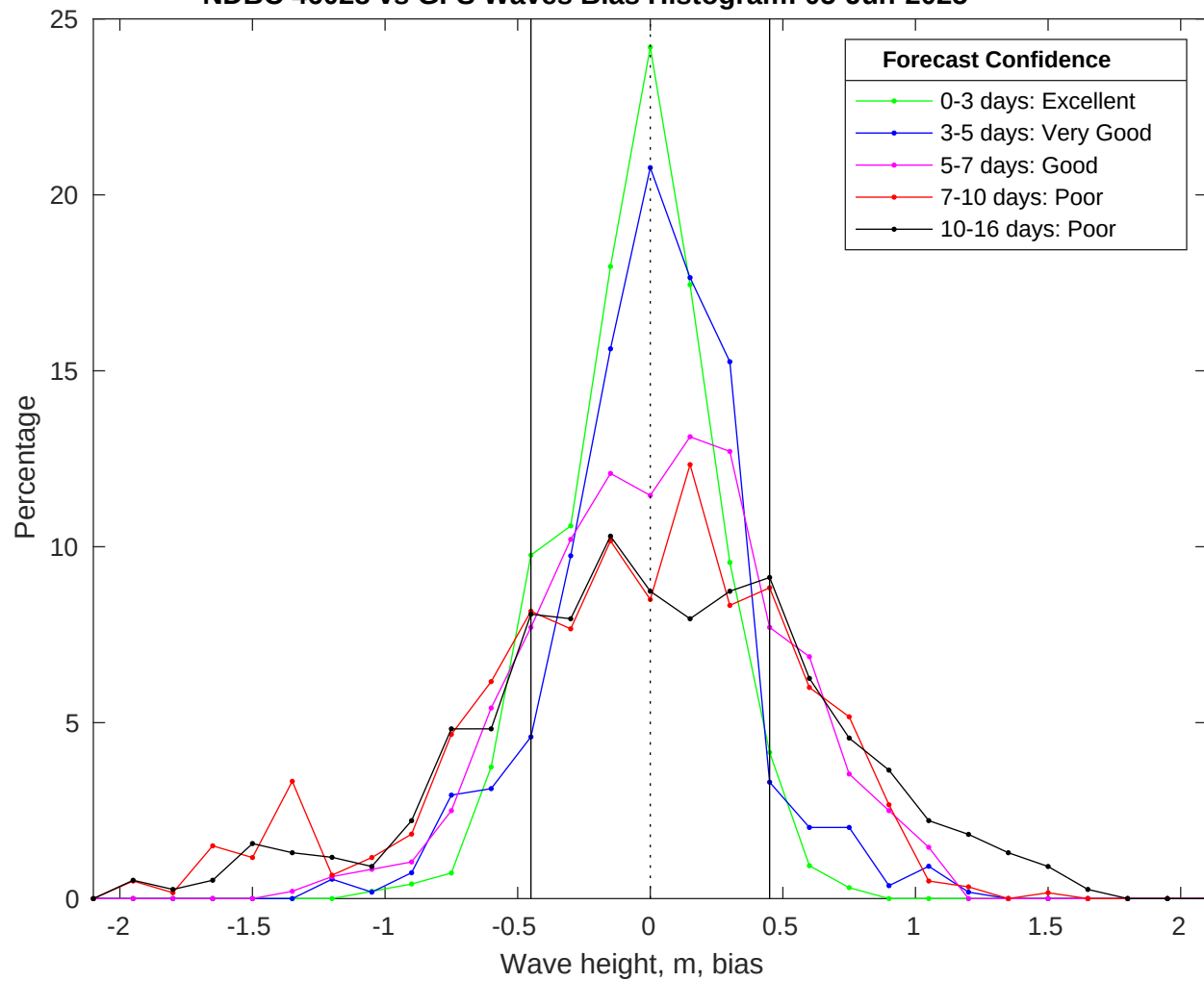
NDBC 46028 vs GFS Waves Bias Histogram: 05-Jun-2025
