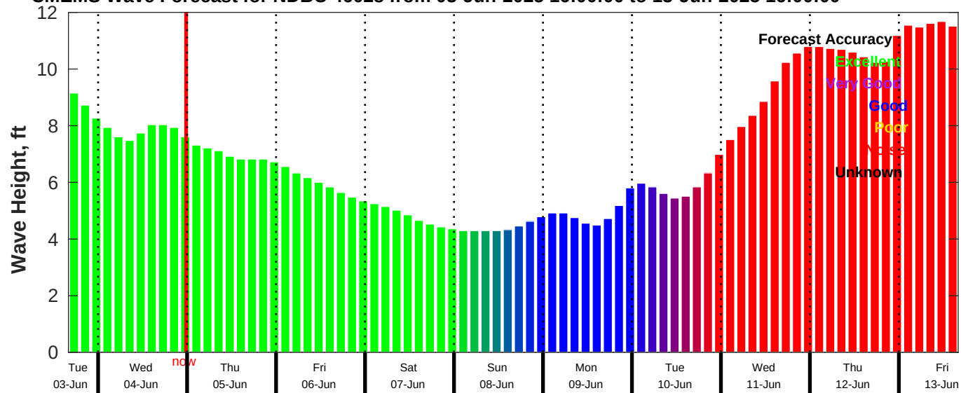
CMEMS Wave Forecast for NDBC 46028 from 03-Jun-2025 16:00:00 to 13-Jun-2025 16:00:00
