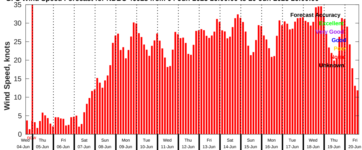
GFS Wind Speed Forecast for NDBC 46028 from 04-Jun-2025 16:00:00 to 20-Jun-2025 16:00:00
