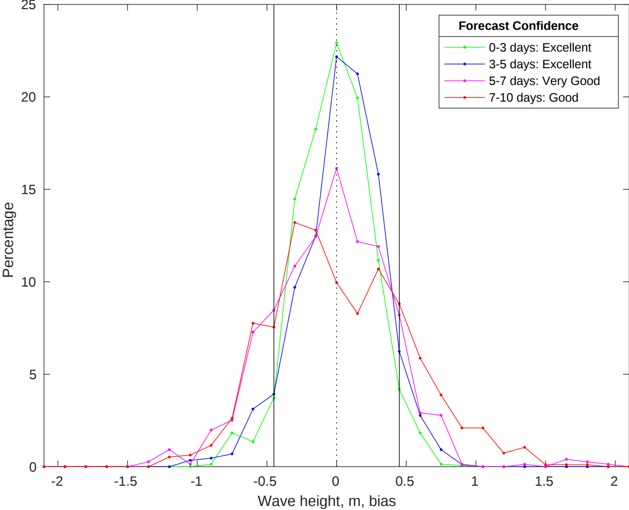
NDBC 46054 vs CMEMS Waves Bias Histogram: 05-Jun-2025
