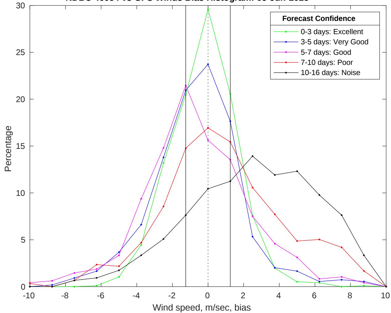
NDBC 46054 vs GFS Winds Bias Histogram: 05-Jun-2025
