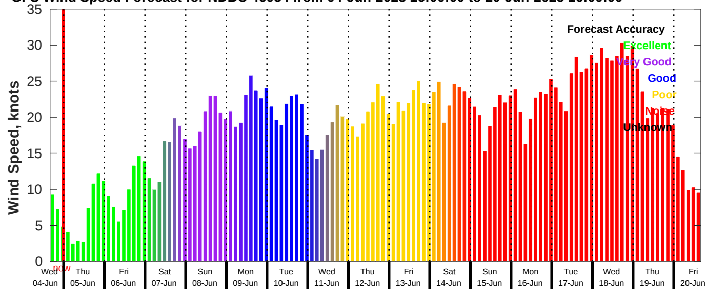
GFS Wind Speed Forecast for NDBC 46054 from 04-Jun-2025 16:00:00 to 20-Jun-2025 16:00:00
