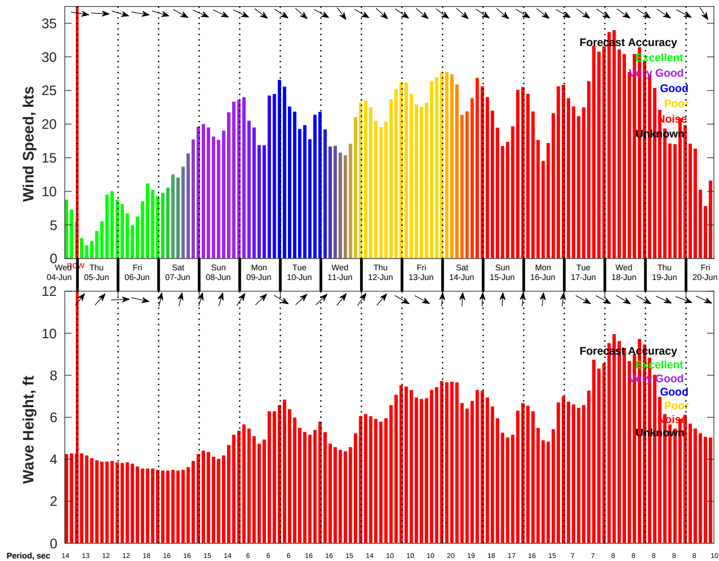
Wind & Wave Forecast for NDBC 46069 from 04-Jun-2025 16:00:00 to 20-Jun-2025 16:00:00
