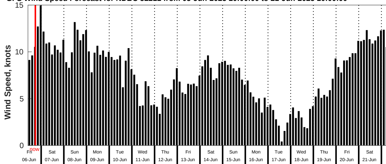
GFS Wind Speed Forecast for NDBC 52211 from 05-Jun-2025 10:00:00 to 21-Jun-2025 10:00:00
