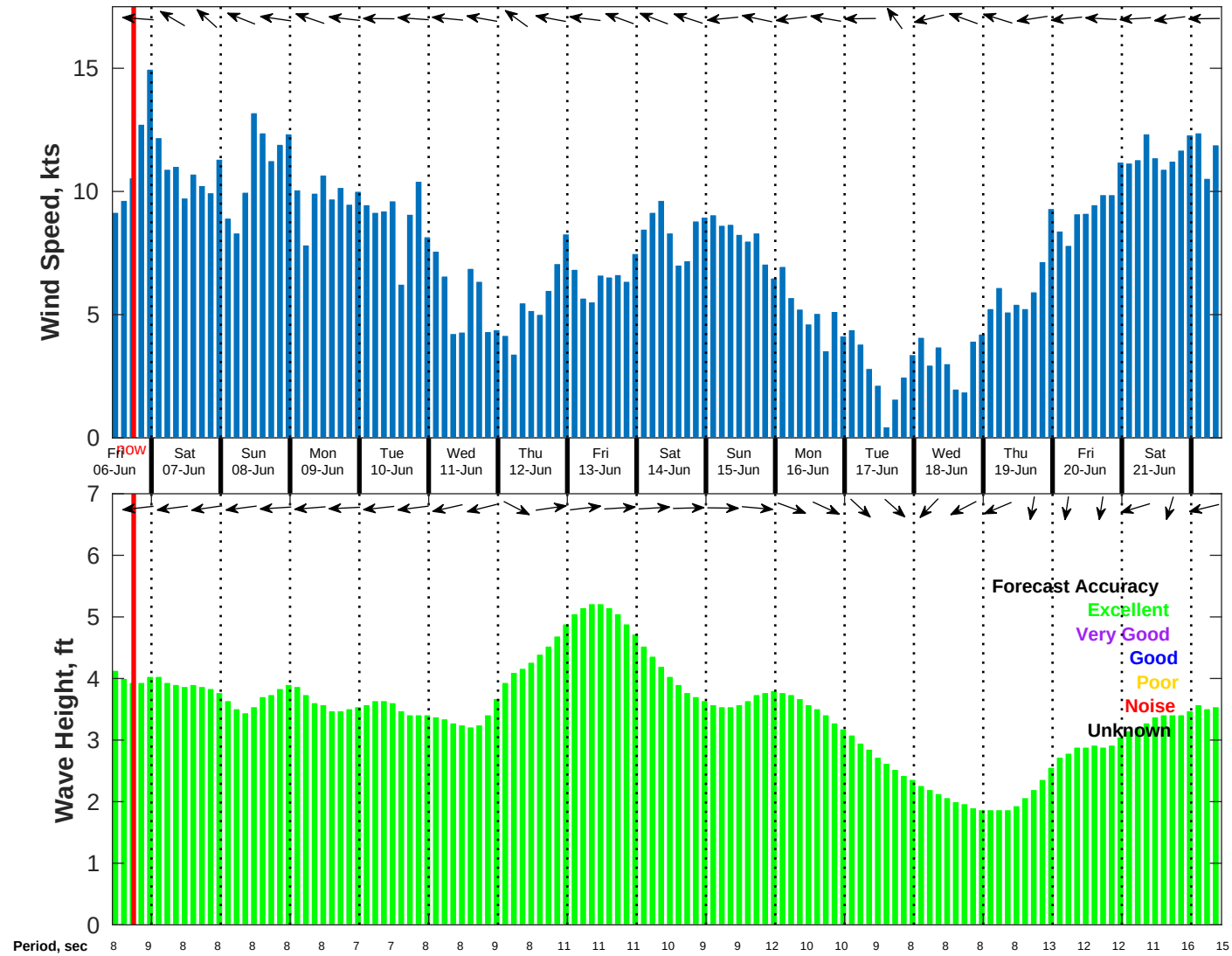
Wind & Wave Forecast for NDBC 52211 from 05-Jun-2025 10:00:00 to 21-Jun-2025 10:00:00
