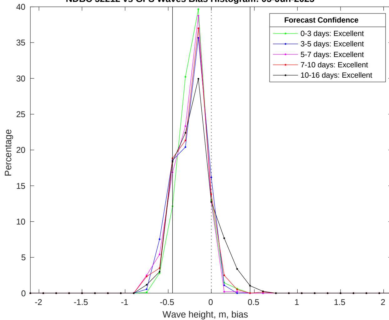
NDBC 52212 vs GFS Waves Bias Histogram: 05-Jun-2025
