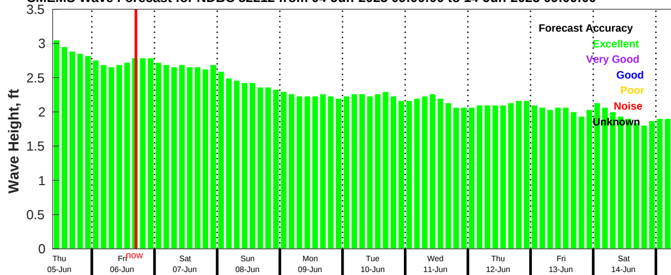
CMEMS Wave Forecast for NDBC 52212 from 04-Jun-2025 09:00:00 to 14-Jun-2025 09:00:00
