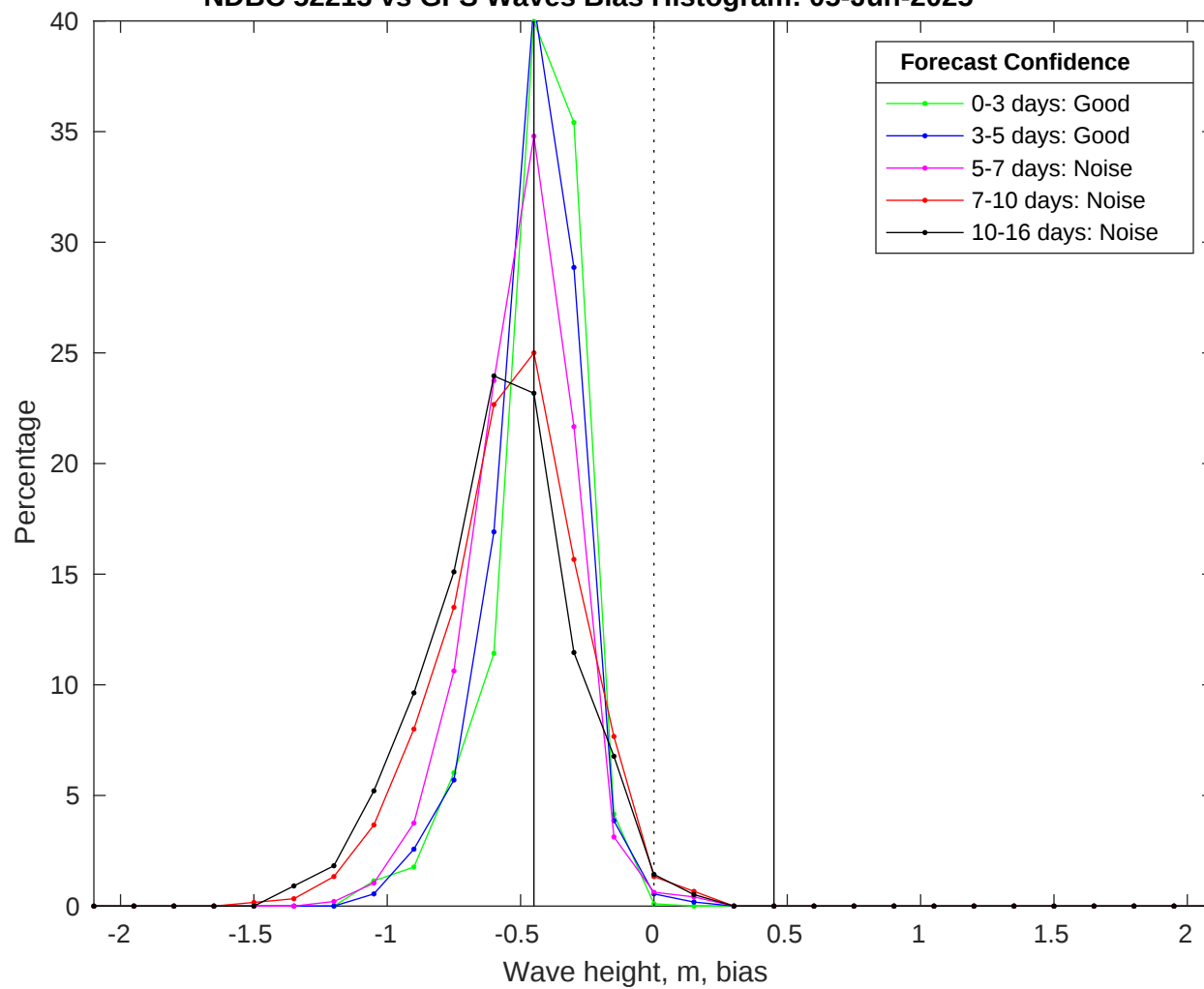
NDBC 52213 vs GFS Waves Bias Histogram: 05-Jun-2025
