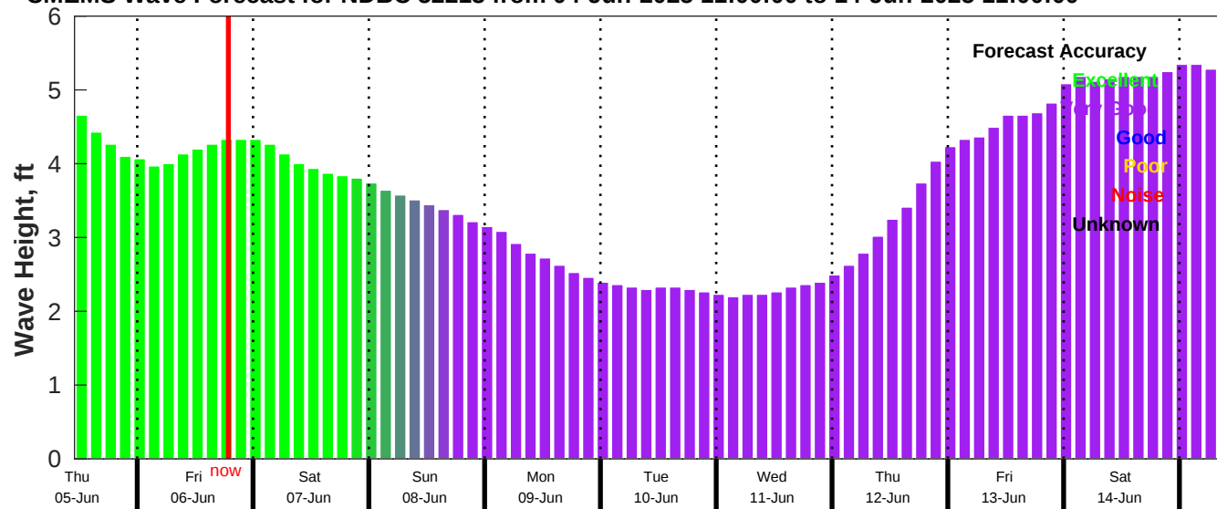
CMEMS Wave Forecast for NDBC 52213 from 04-Jun-2025 11:00:00 to 14-Jun-2025 11:00:00
