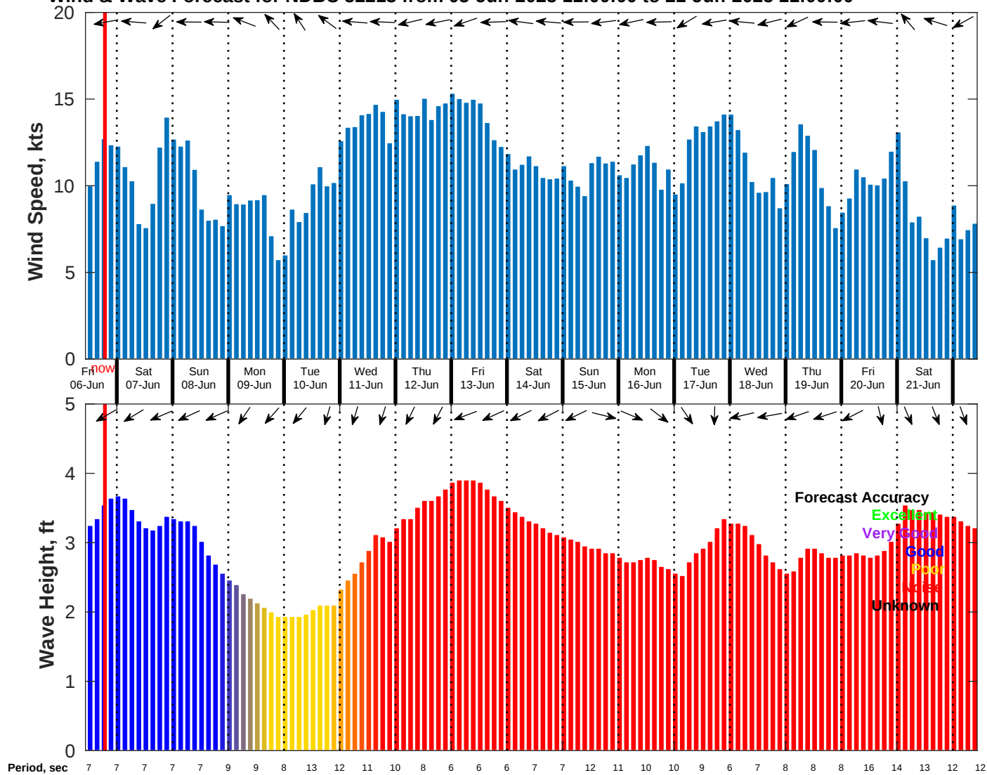
Wind & Wave Forecast for NDBC 52213 from 05-Jun-2025 11:00:00 to 21-Jun-2025 11:00:00
