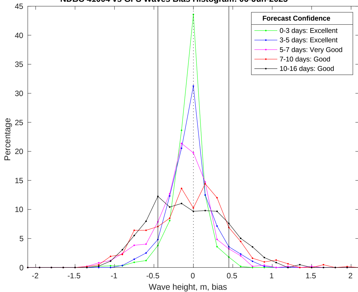
NDBC 41004 vs GFS Waves Bias Histogram: 06-Jun-2025
