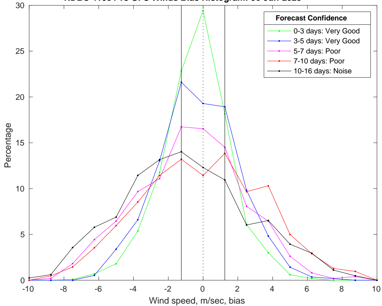
NDBC 41004 vs GFS Winds Bias Histogram: 06-Jun-2025
