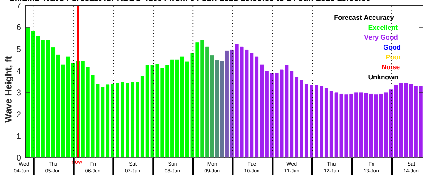
CMEMS Wave Forecast for NDBC 41004 from 04-Jun-2025 19:00:00 to 14-Jun-2025 19:00:00
