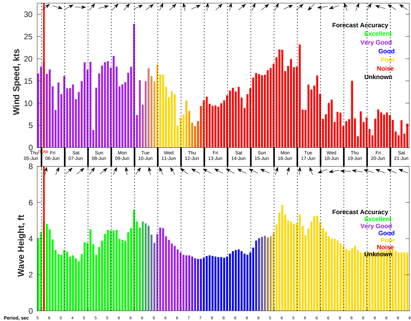
Wind & Wave Forecast for NDBC 41004 from 05-Jun-2025 19:00:00 to 21-Jun-2025 19:00:00
