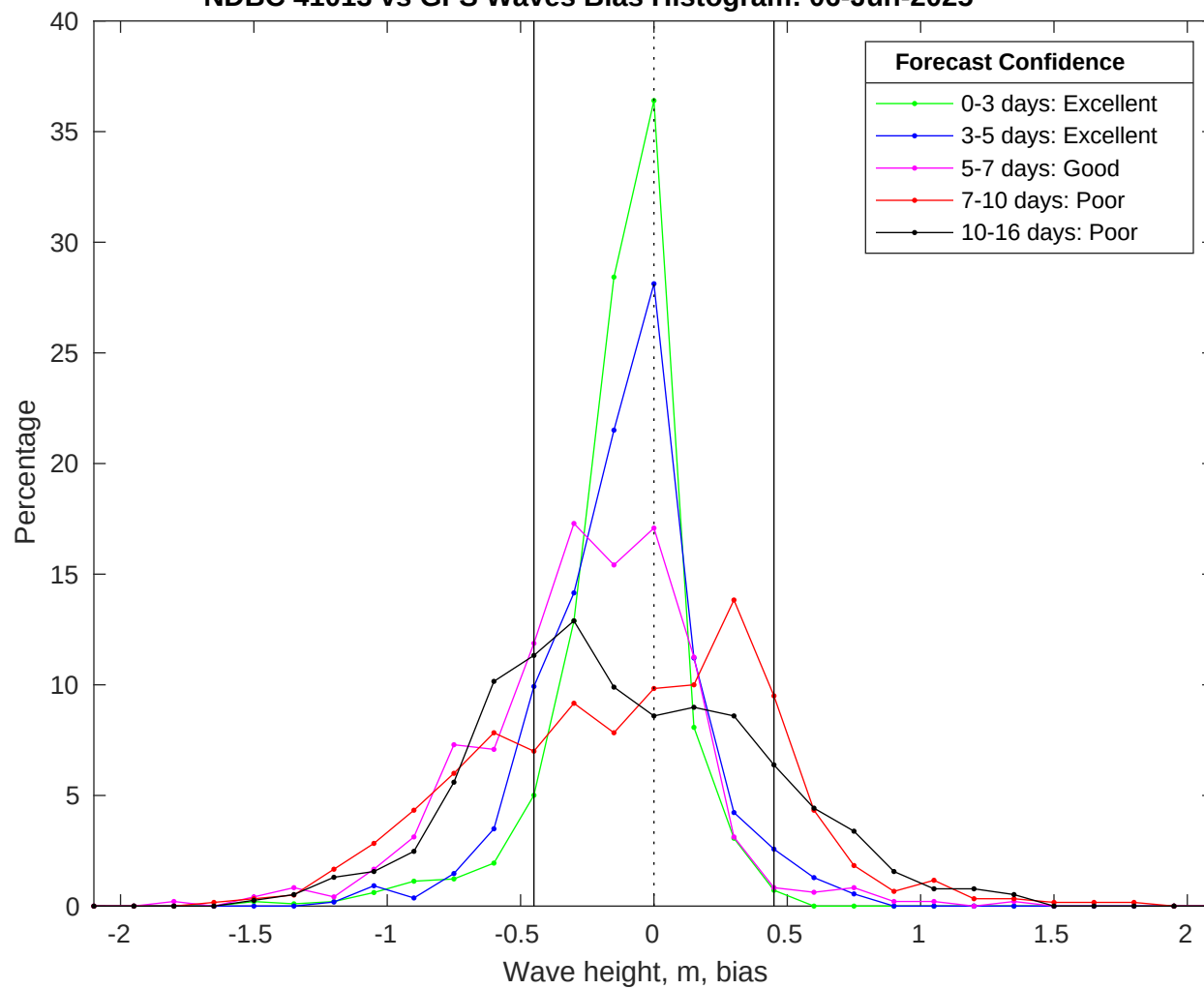
NDBC 41013 vs GFS Waves Bias Histogram: 06-Jun-2025
