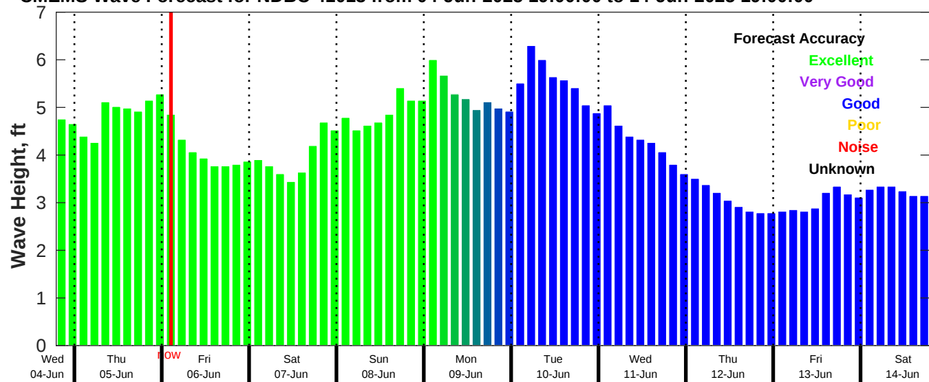
CMEMS Wave Forecast for NDBC 41013 from 04-Jun-2025 19:00:00 to 14-Jun-2025 19:00:00
