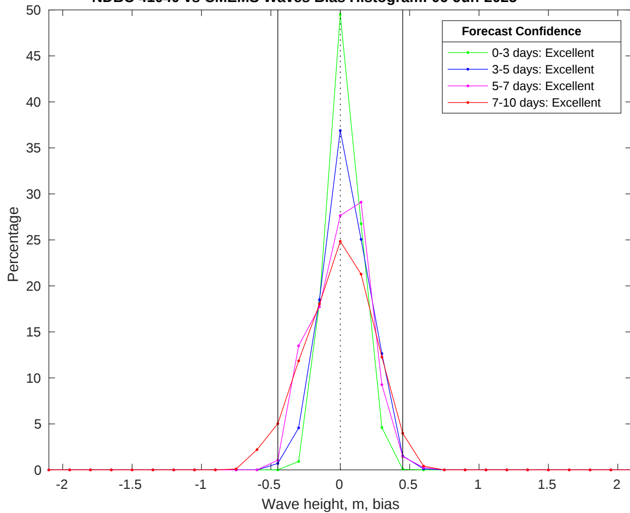
NDBC 41040 vs CMEMS Waves Bias Histogram: 06-Jun-2025
