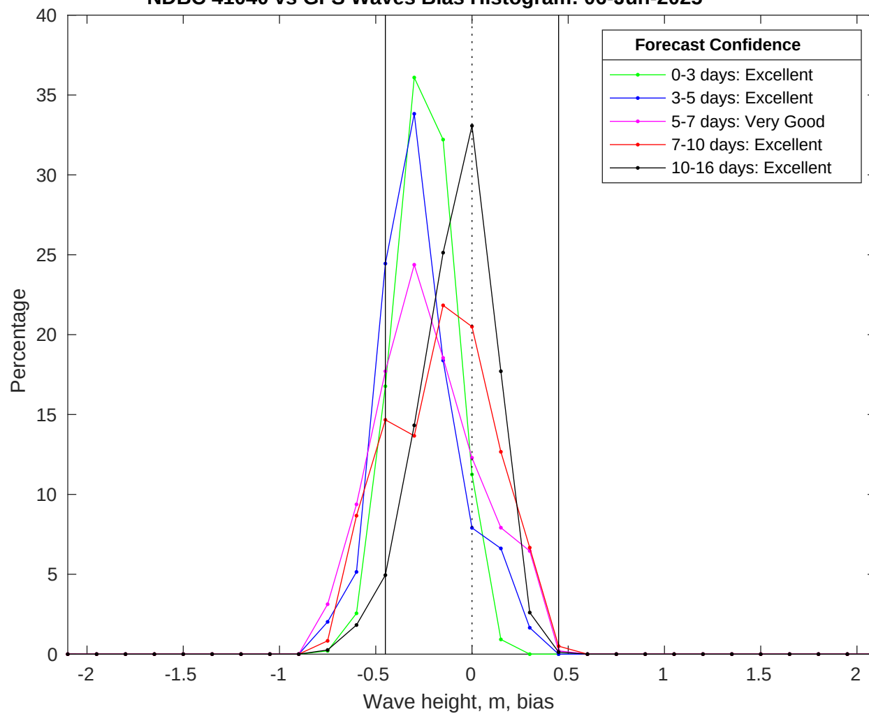
NDBC 41040 vs GFS Waves Bias Histogram: 06-Jun-2025
