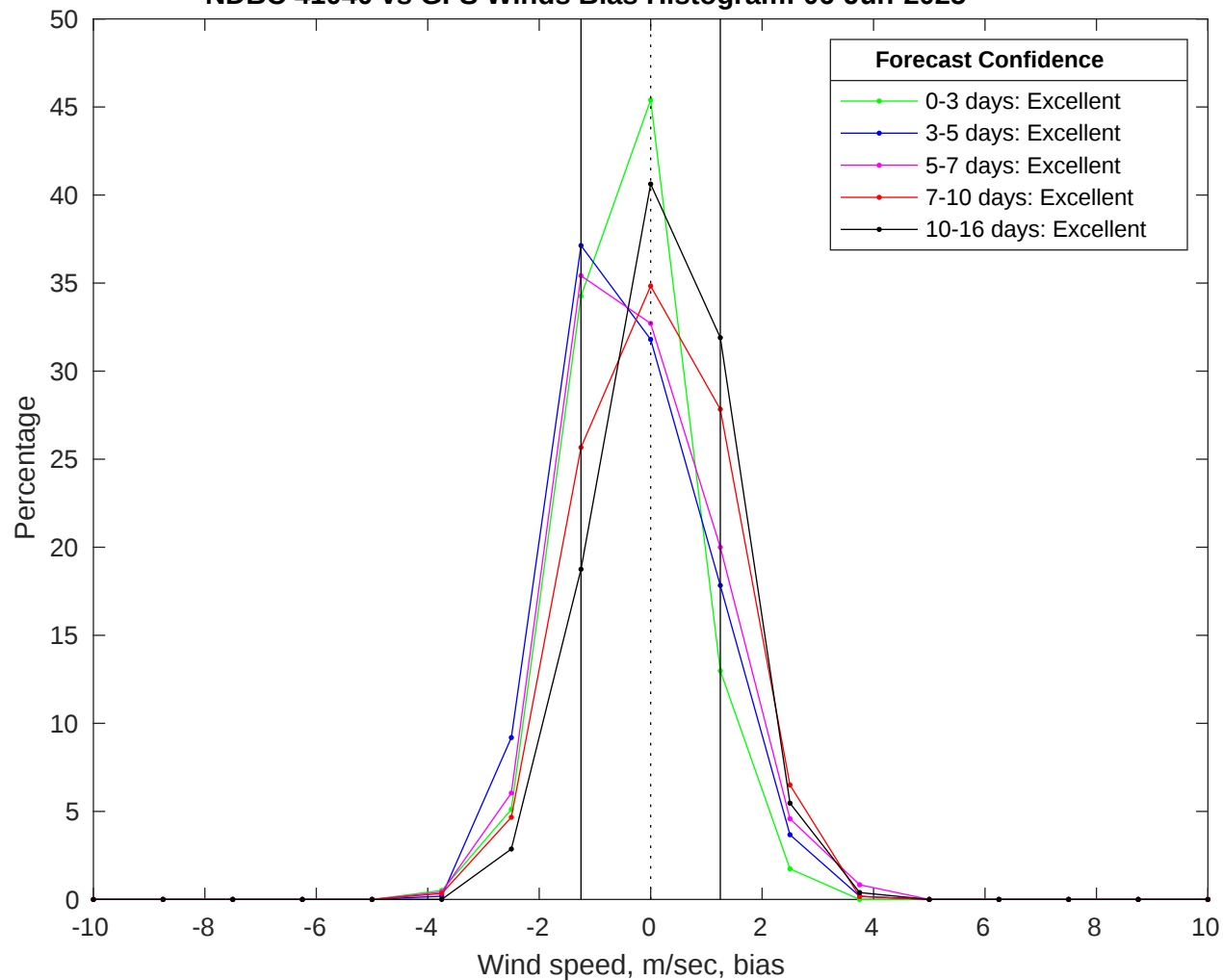
NDBC 41040 vs GFS Winds Bias Histogram: 06-Jun-2025
