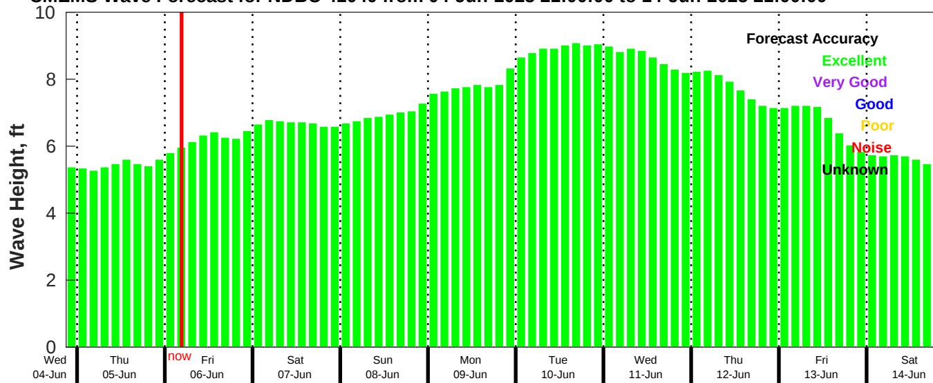
CMEMS Wave Forecast for NDBC 41040 from 04-Jun-2025 21:00:00 to 14-Jun-2025 21:00:00
