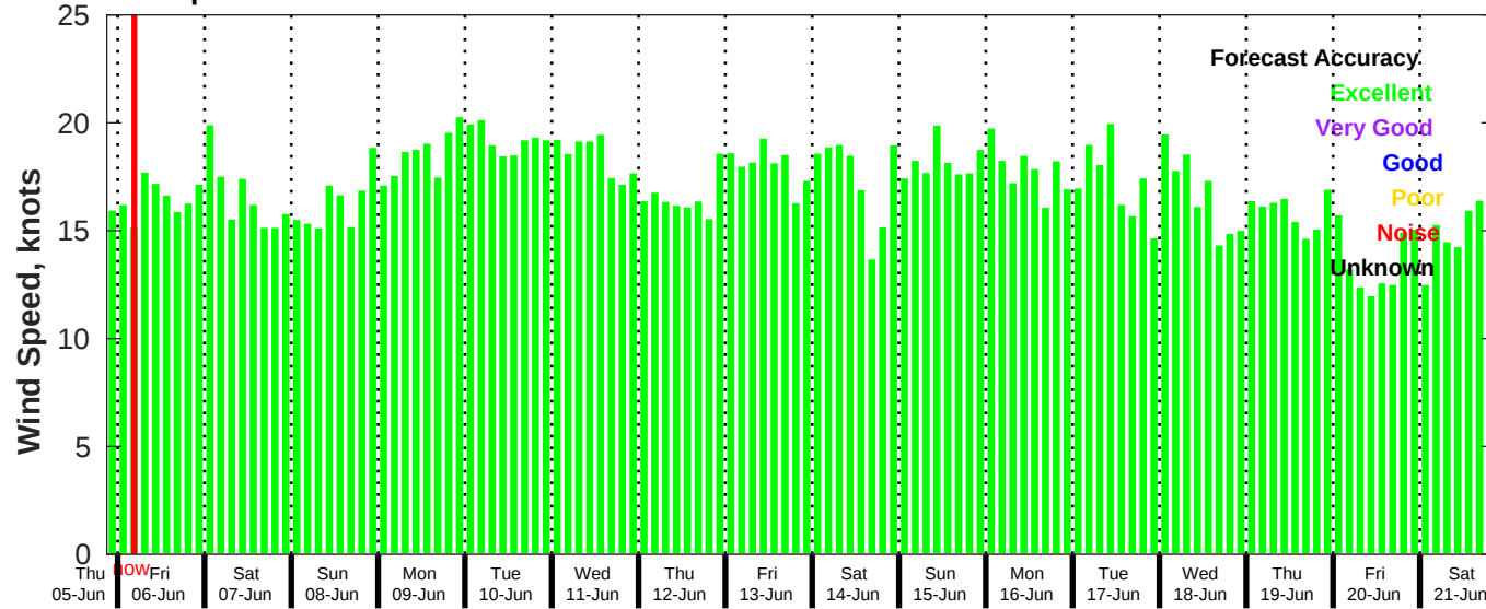
GFS Wind Speed Forecast for NDBC 41040 from 05-Jun-2025 21:00:00 to 21-Jun-2025 21:00:00
